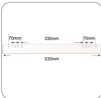
Wall mount bracket measurements
